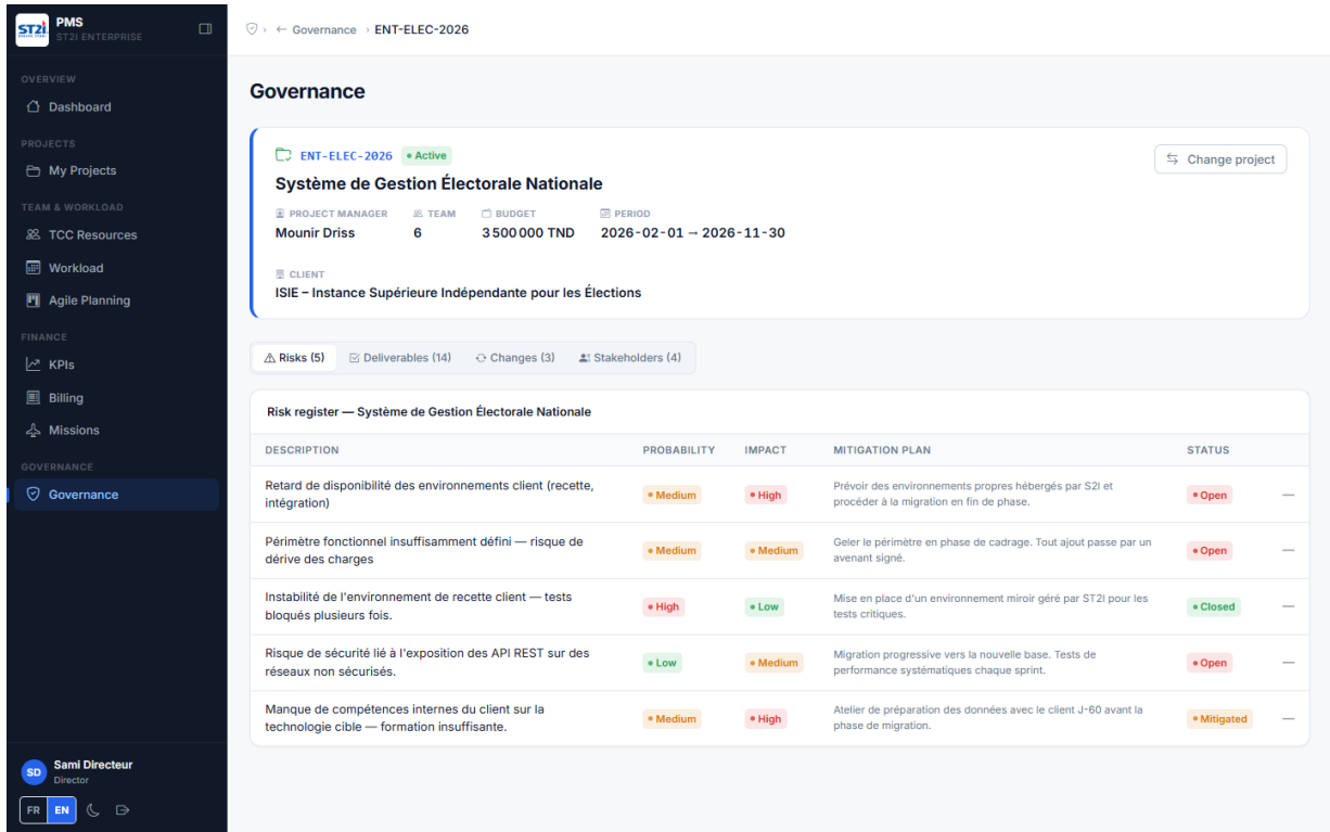
Figure 6.7: Governance interface
