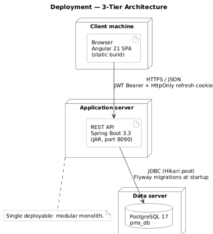
Figure 3.7: Deployment architecture
