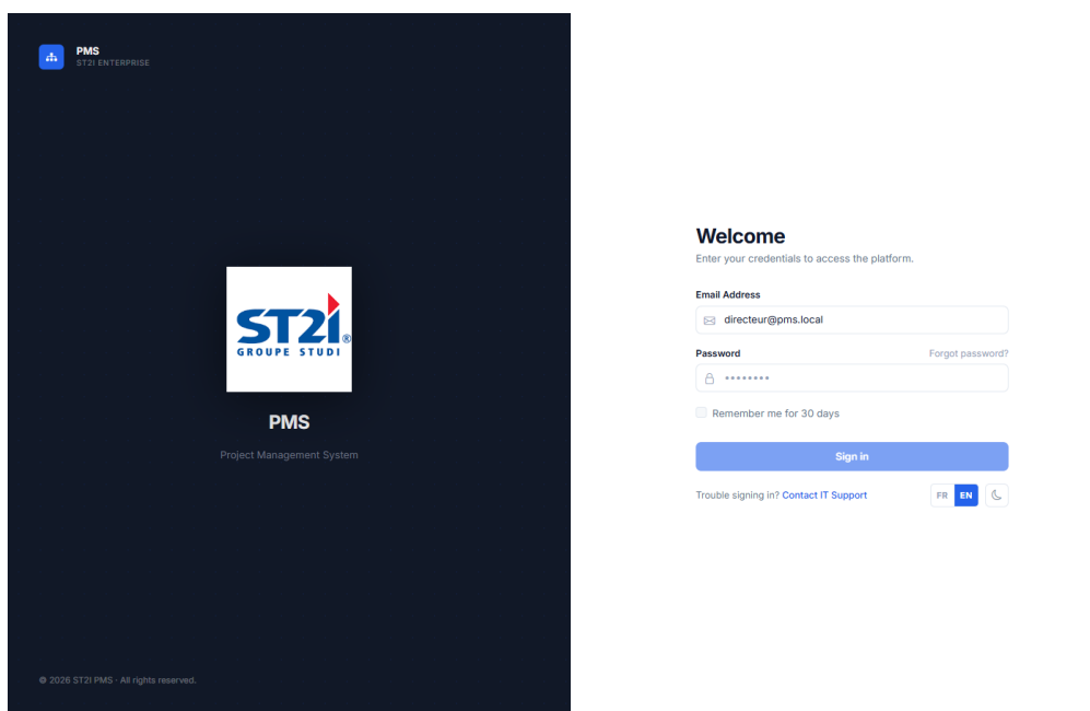
Figure 4.13: Login interface
